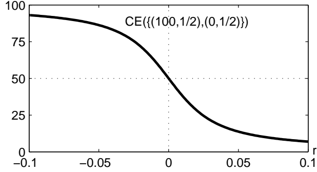
Figure 4: Certainty equivalent of a simple gamble as a function of the risk-aversity.
