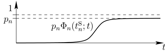
Figure 3: Unconditional distribution for successful completion probability.
