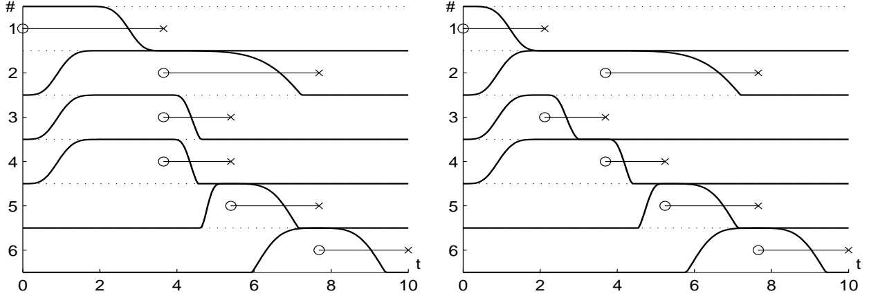
Figure 8: CE(t_n^s) graphs for the corresponding reasonable schedules in Figure 5.
